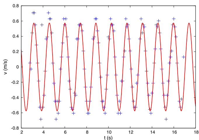
Figure 6. Velocity of the smartphone versus time for the data obtained from the simple harmonic motion. Blue crosses represent the experimental data, and the red curve the fit.
