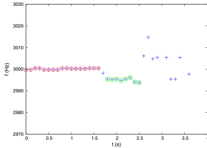
Figure 4. Frequency versus time in a uniform linear motion. Red circles represent the mobile phone at rest, and the green boxes show when it moved away from the source.
