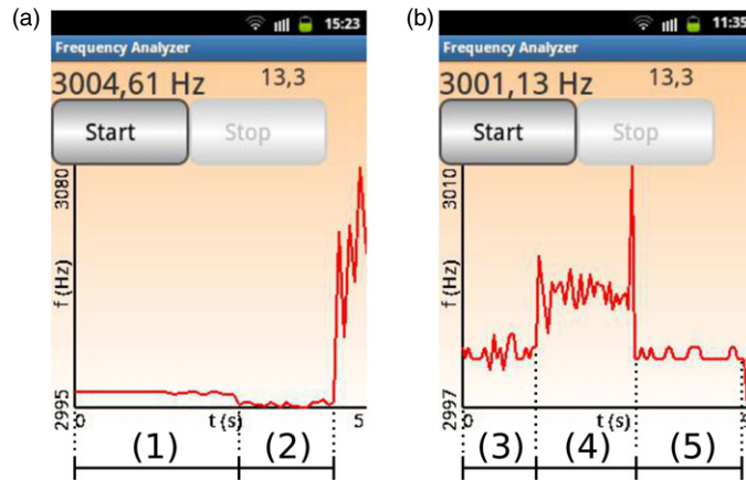
Figure 2. Snapshots of the Frequency Analyzer application for two measurements of the frequency when the smartphone moves with uniform motion on the air track: (a) moving away from the speaker and (b) approaching the speaker.
