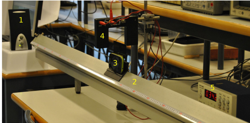
Figure 1. Photograph of the experimental setup used to measure the frequency of a linear motion. In the figure, (1) is the speaker, (2) the air track, (3) the smartphone, (4) the photodetector and (5) the time counter.
