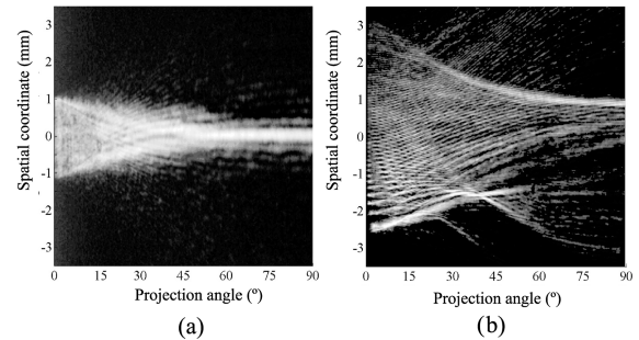
Fig. 3. Experimental Radon-Wigner spectrum of (a) a single slit of 2.2 mm and (b) a binary grating with a linearly increasing spatial frequency.
